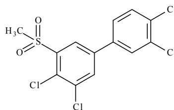
5-methyl-sulfonyl-3,3',4,4'-tetrachlorobiphenyl (methyl sulfone metabolite)
